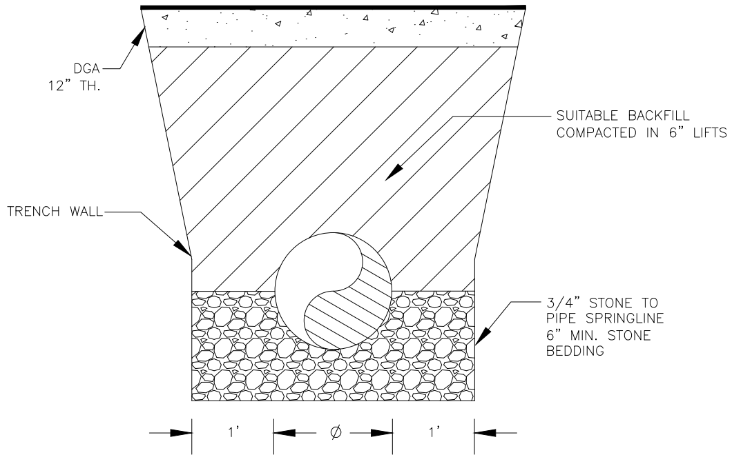
GRAVITY MAIN DETAIL
