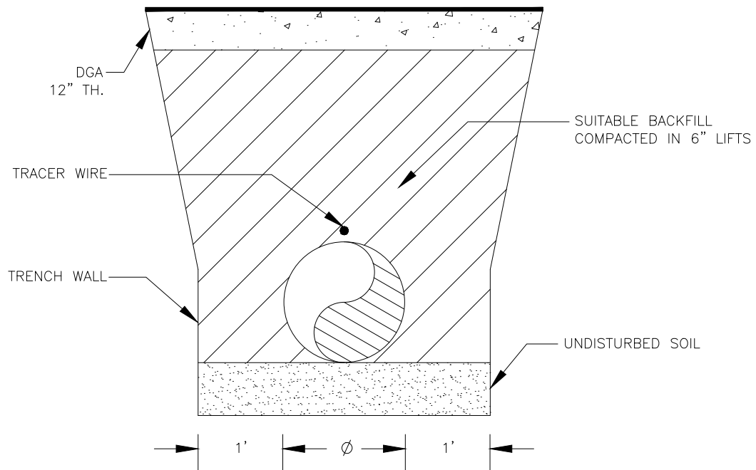
FORCE MAIN DETAIL
