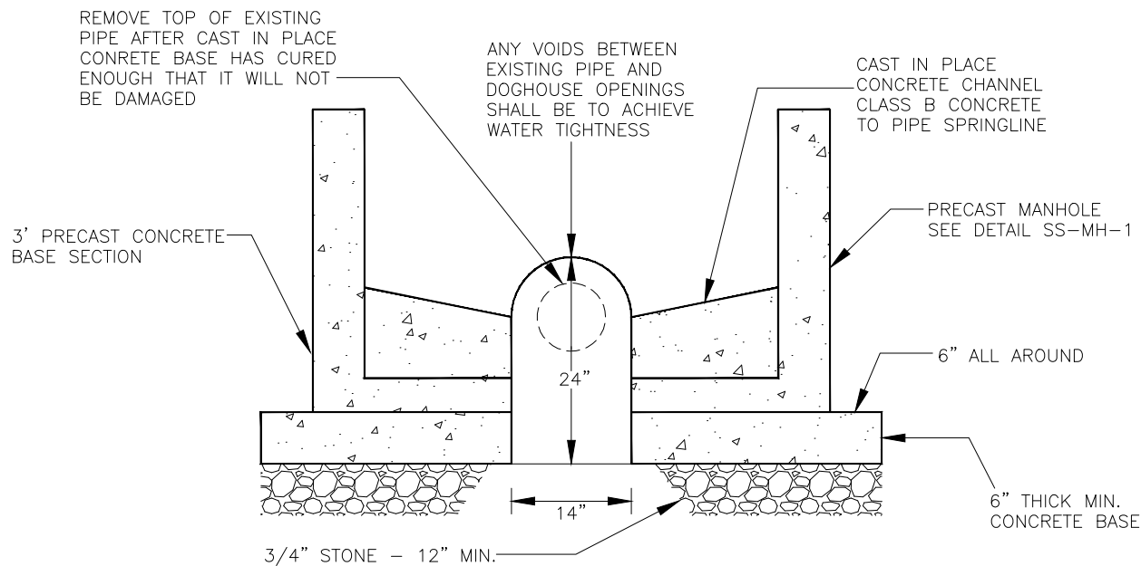
CROSS SECTION
